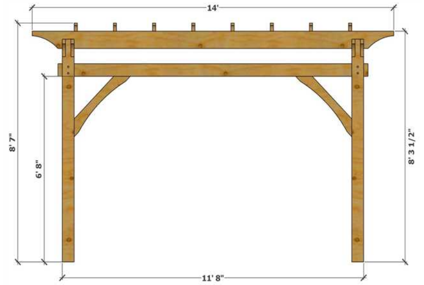
SIDE VIEW
